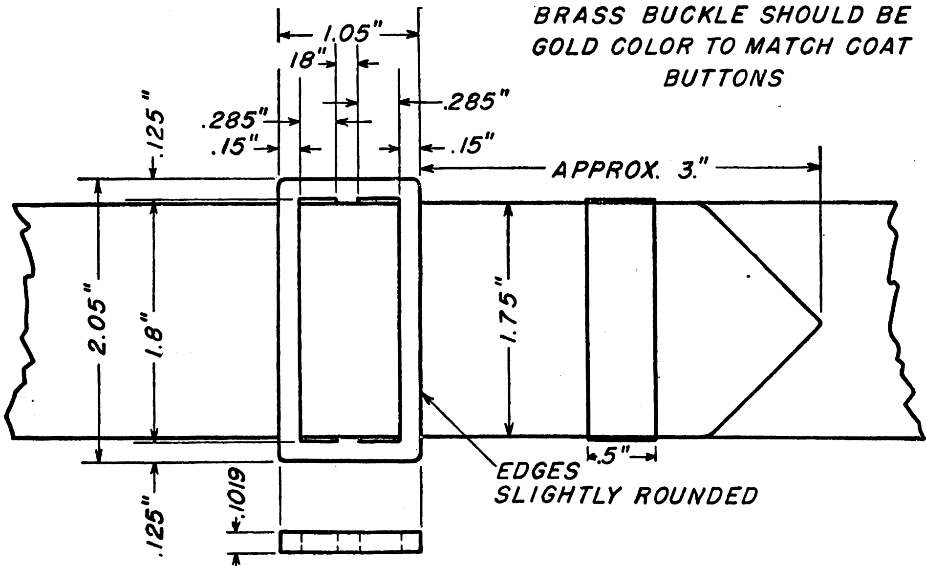
FIGURE 50.— Cloth belt for use on officers' service coat in lieu of officers' belt, M1921.
